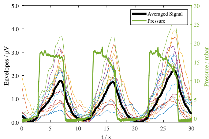
Fig. 13. Envelopes of all 16 EMG signals over three inspiration periods. The bold black plot represents the combined average signal of these envelopes.
