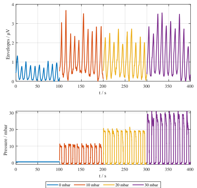
Fig. 15. Averaged envelopes for four different configurations of the inspiration pressure valve. Below, the corresponding measured pressure is plotted. The subject sat on a chair during the measurement.
