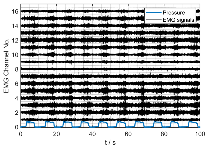
Fig. 10. EMG channels 1-16 during 10 respiratory cycles. The time periods of inspiration can be seen in the blue pressure plot below.
