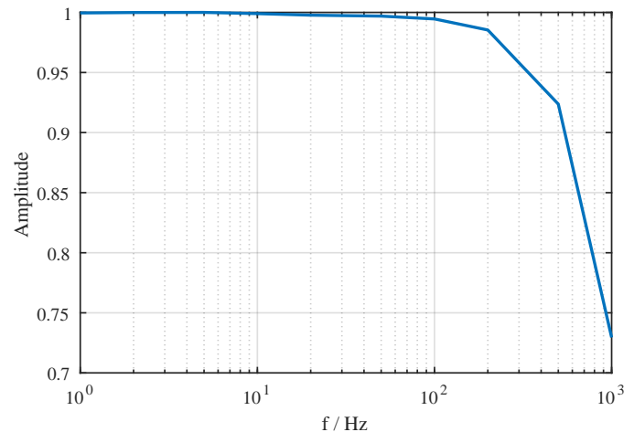
Fig. 8. Measured magnitude response of the EMG channels.
