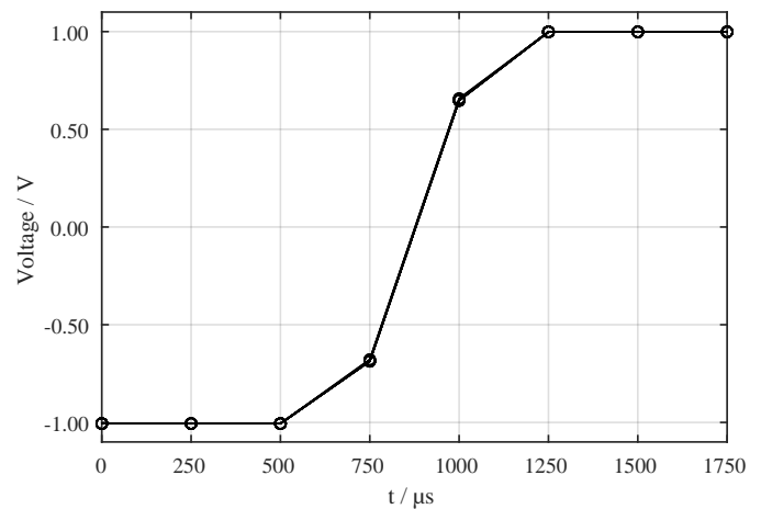
Fig. 7. Measured step responses from -1 V to 1 V of all 16 EMG channels. Caused by the synchronous digitization of all channels, timing differences between these 16 plots can hardly be seen.
