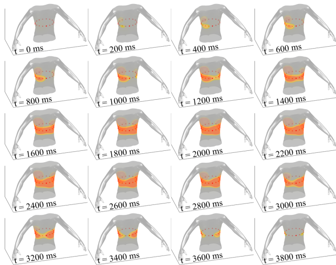
Fig. 12. 3-dimensional representation of the EMG measurement results during inhalation.
