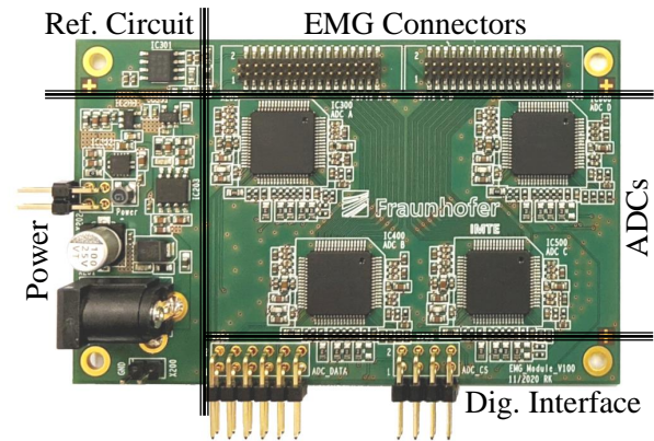
Fig. 4. Photograph of the system's EMG analog front end PCB. In this study, only two ADCs with eight channels each are used.
