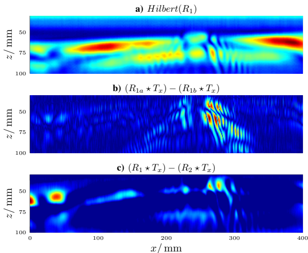
Fig. 9. Acoustic profiles of a copper cylinder (6 mm diameter) on an acrylic plate.
