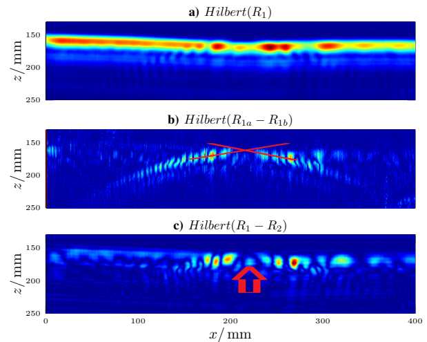
Fig. 10. Acoustic profiles of a copper cylinder (6 mm diameter) on an absorber plate.
