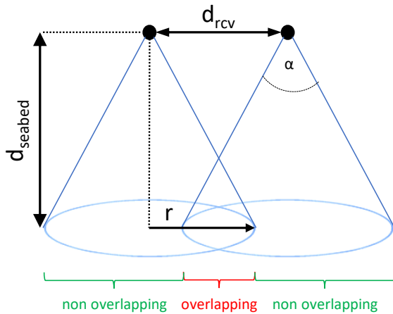
Fig. 6. Beam radius and overlapping in differential setup
