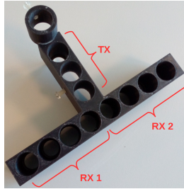
Fig. 3. Mounting system for differential measurement
